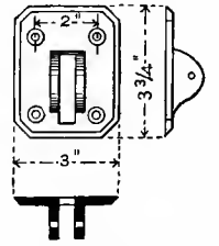
Figs. 4267-4269. BERTH-CATCH.
